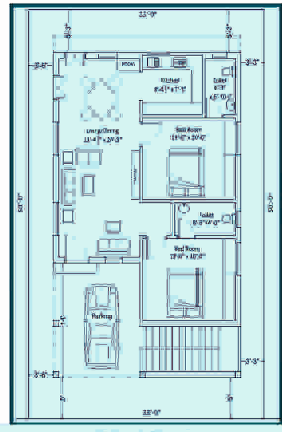
GROUND FLOOR PLAN 1095.00 SQ FTS SLAB AREA 940.00 SQ FTS PLINTH AREA
